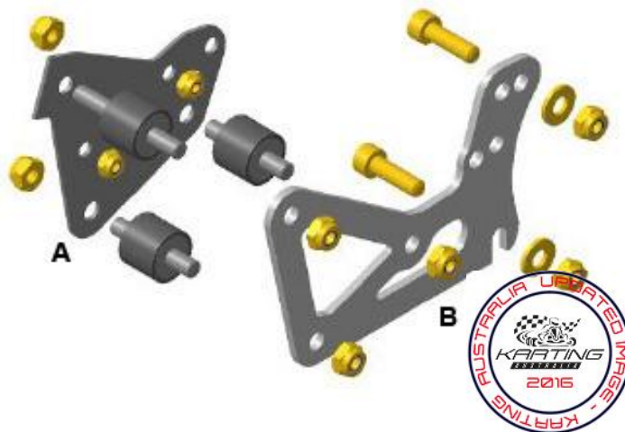
Support Plate System for Rotax 125 Micro MAX
