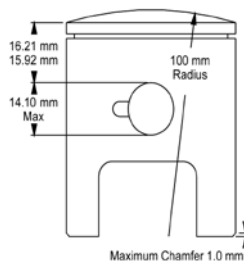
DIAGRAM IS FOR DIMENSIONAL REFERENCE ONLY.
